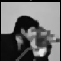
\alpha=3.2e-02 | T=1.0e-03
