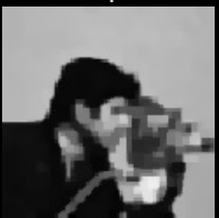
\alpha=1.0e-02 | T=1.0e-03
