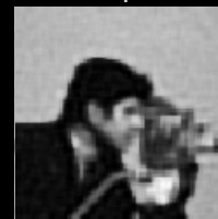
\alpha=1.0e-02 | T=1.0e-01
